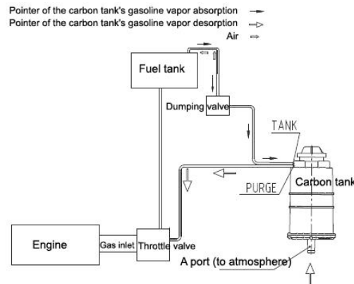
Fuel evaporation control system diagram
